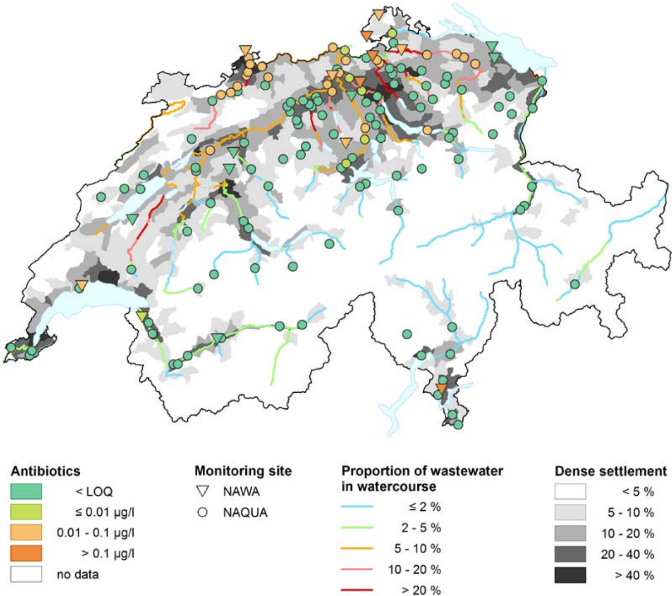
Figure 2: Antibiotics in groundwater and river water in relation to percentage of wastewater in selected rivers. Monitoring sites are part of the NAQUA (National Groundwater Monitoring) and the NAWA (National Surface Water Monitoring Network). Rivers with a discharge Q347 >2000 l/s are plotted.
